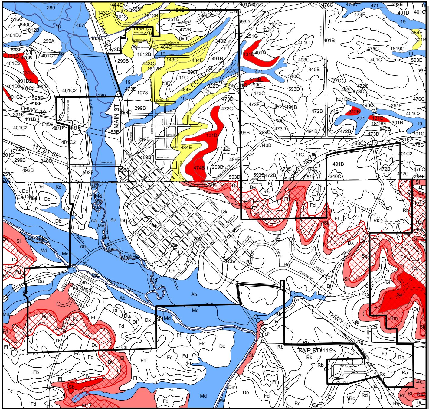
FIG. #25 SOIL MAP
